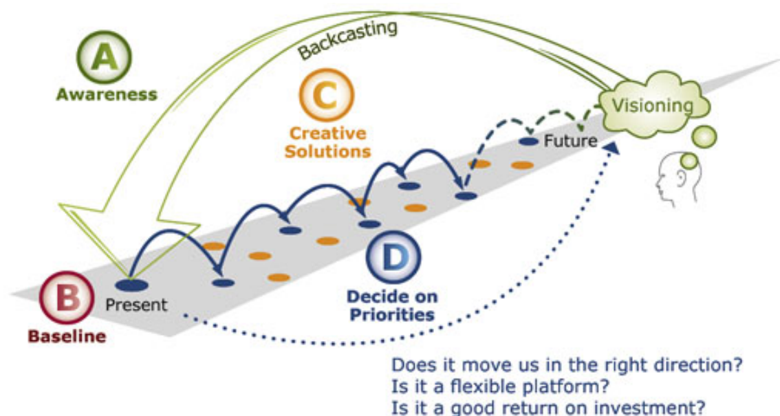
Figure 4: Backcasting
